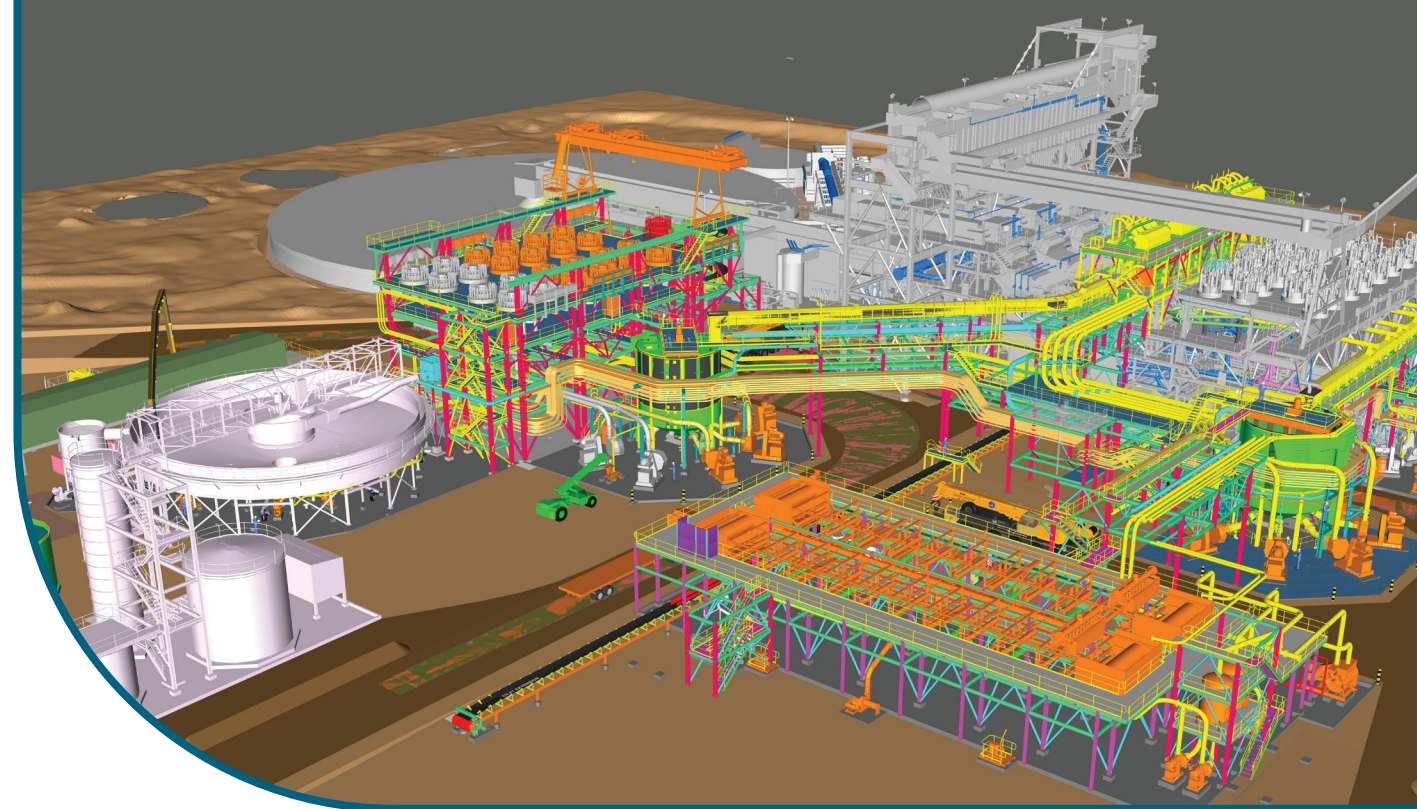
Image: PBO Tertiary Hydrocyclones Plant — Pilbara, WA.
