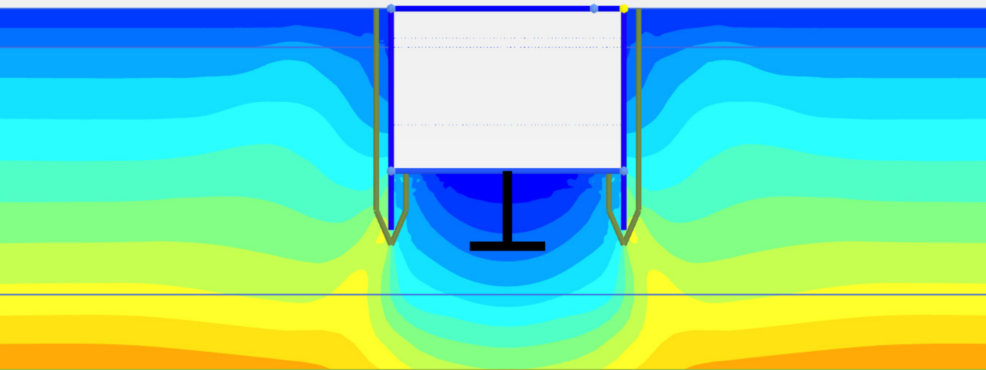
Image: PmaxP Lease 11 Track Unloader PLAXIS 2D Analysis Model.
