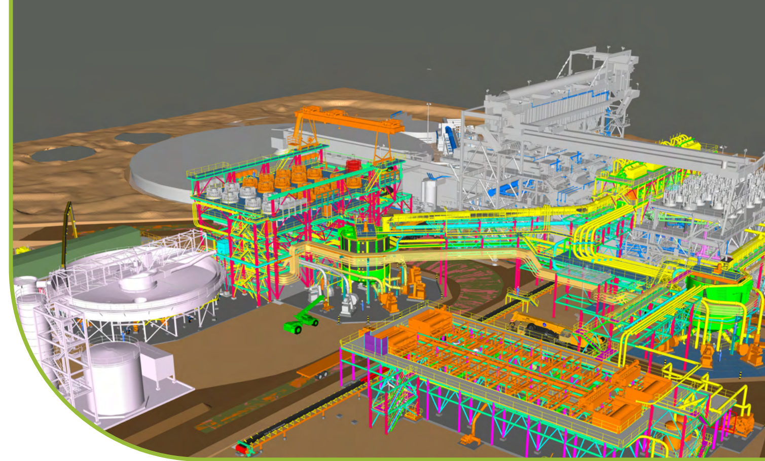
Image: PBO Tertiary Hydrocyclones Plant — Pilbara, WA.
